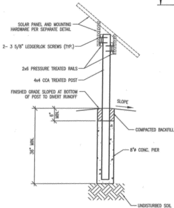
FOUNDATION SECTION
